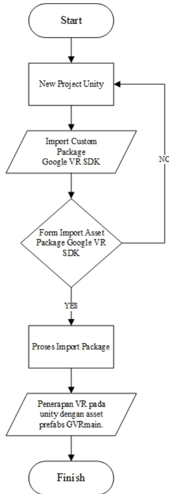
Gambar 8. Flowchart Implementasi Google VR SDK
